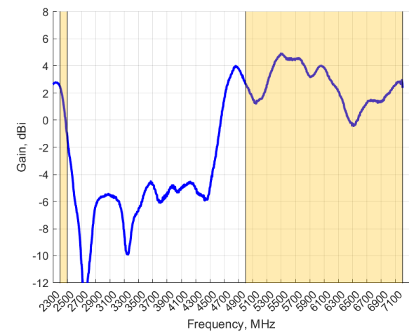
GAIN (Excluding Cable Loss): Wi-Fi Antenna
