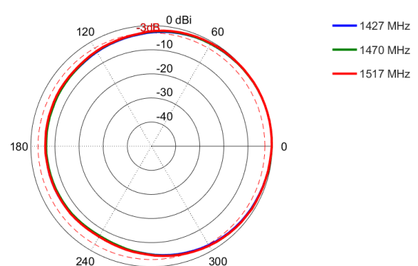
Azimuth: 1427 – 1517 MHz
