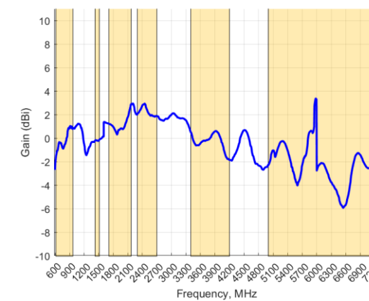
GAIN (EXCLUDING CABLE LOSS): Cellular Horizontal
