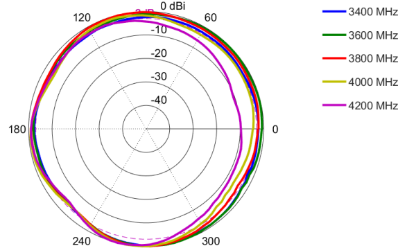
Azimuth: 3400 – 4200 MHz
