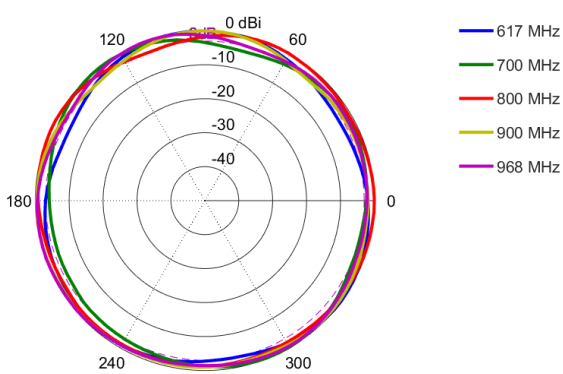
Azimuth: 617 – 968 MHz
