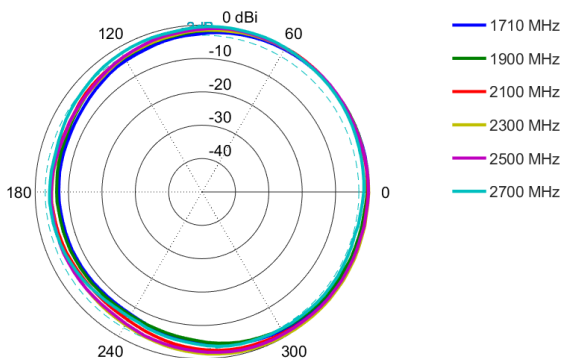
Azimuth: 1710 – 2700 MHz
