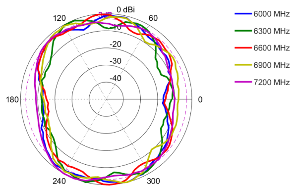
Azimuth: 6000 – 7200 MHz
