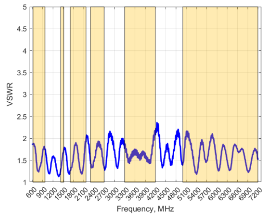
VSWR: Cellular Vertical
