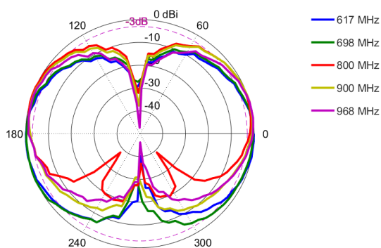
Elevation: 617 – 968 MHz
