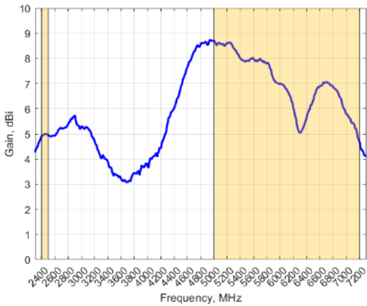
GAIN (EXCLUDING CABLE LOSS): WI-FI
