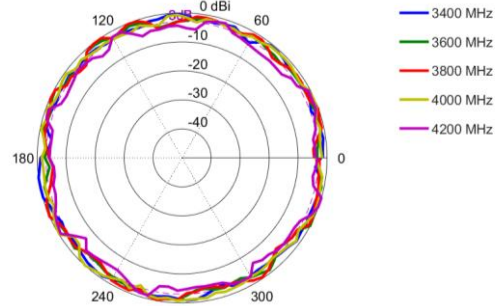
Azimuth: 3400 – 4200 MHz
