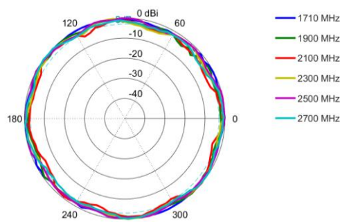
Azimuth: 1710 – 2700 MHz
