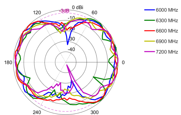
Elevation: 6000 – 7200 MHz
