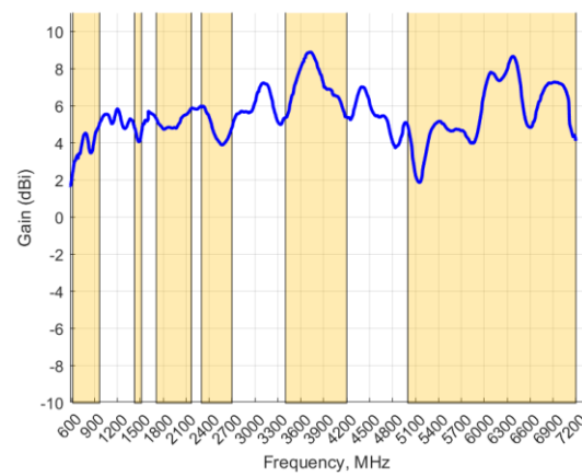
GAIN (EXCLUDING CABLE LOSS): Cellular Vertical
