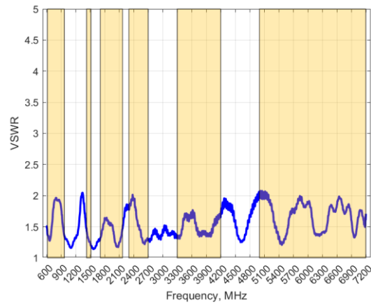
VSWR: Cellular Horizontal
